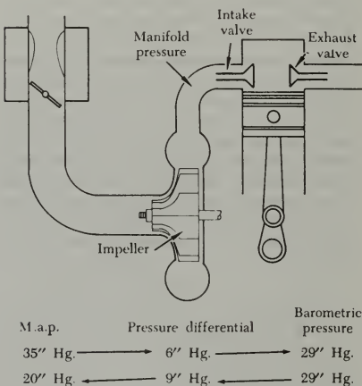
FIGURE 10-40. Effect of valve overlap.
